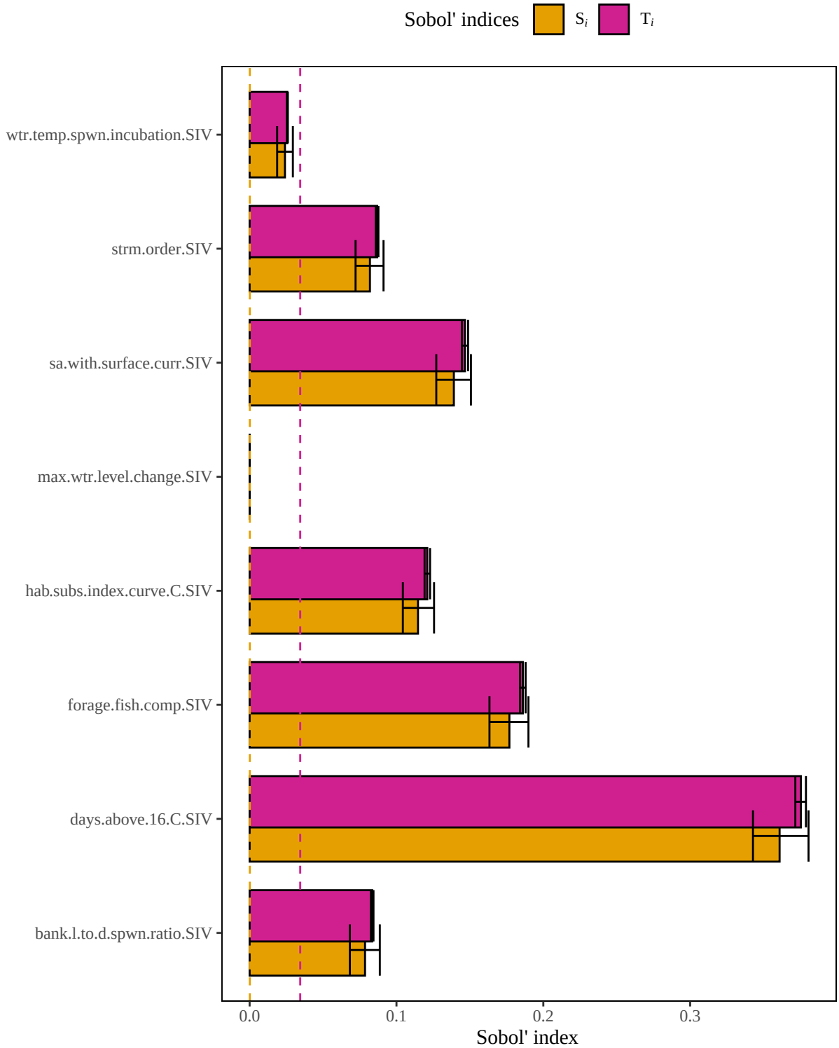
Figure 5. Results of a sensitivity analysis for the whitebassRivCurveCSubsIndex model based on a geometric mean structure. Dashed lines represent baseline numerical approximation error for S_i and T_i ( i.e. , dummy variables).
