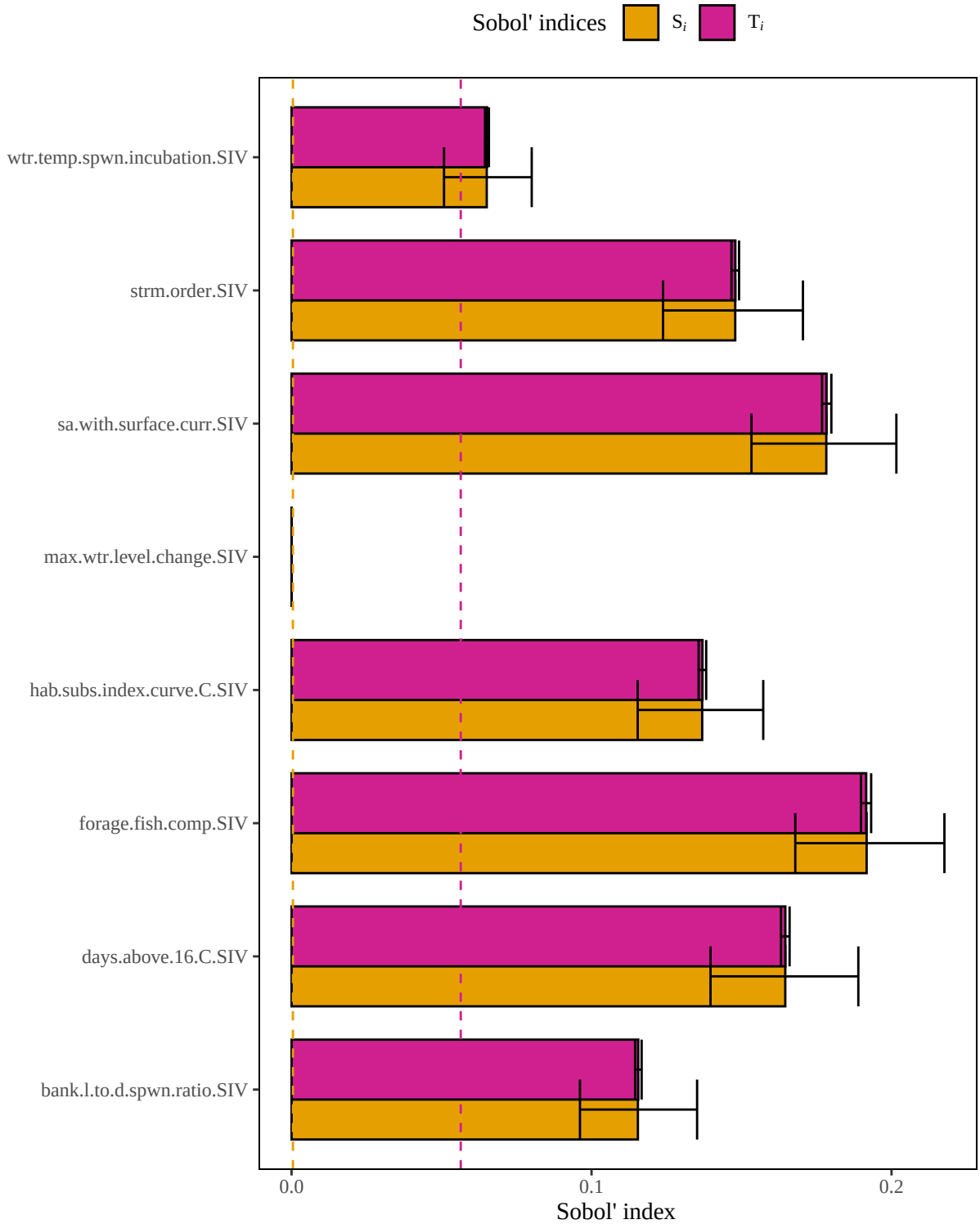
Figure 4. Results of a sensitivity analysis for the whitebassRivCurveCSubsIndex model based on an arithmetic mean structure. Dashed lines represent baseline numerical approximation error for S_i and T_i ( i.e. , dummy variables).
